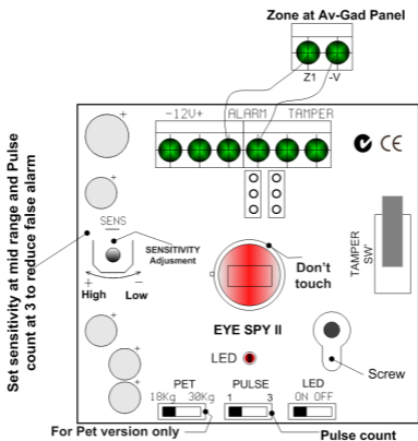
Figure 4: Eye-Spy II PCB layout
