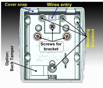
Figure 1: Mounting and wires entry
