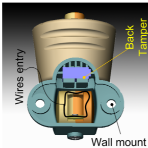
Figure 2: Eye-Spy II bracket (back view)
